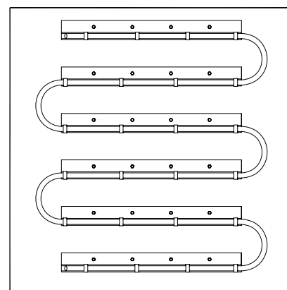
PANEL PIPING 2' x 2' 6 PASS 600 mm x 600 mm
